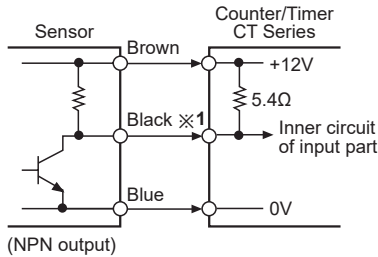
(NPN output)
